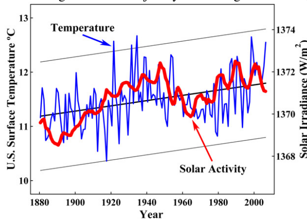
Figure 5: U.S. surface temperature from Figure 4 as compared with total solar irradiance (19) from Figure 3. Between 1900 and 2000, on absolute scales of solar irradiance and degrees Kelvin, solar activity increased 0.19%, while a 0.5 °C temperature change is 0.21%. This is in good agreement with estimates that Earth's temperature would be reduced by 0.6 °C through particulate blocking of the sun by 0.2% (18).
