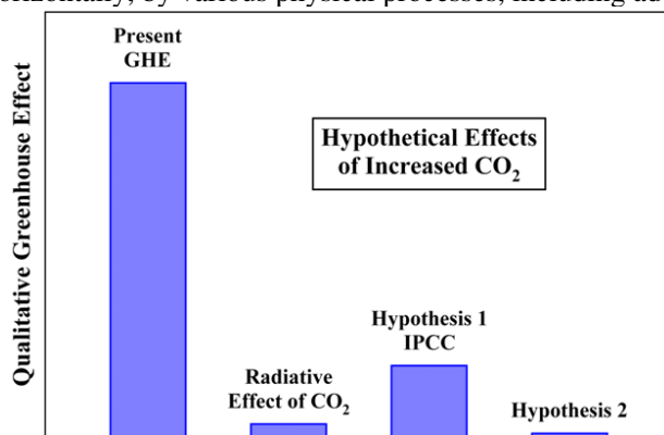
Figure 18: Qualitative illustration of greenhouse warming. "Present GHE" is the current greenhouse effect from all atmospheric phenomena. "Radiative effect of CO 2 " is the added greenhouse radiative effect from doubling CO 2 without consideration of other atmospheric components. "Hypothesis 1 IPCC" is the hypothetical amplification effect assumed by IPCC. "Hypothesis 2" is the hypothetical moderation effect.
